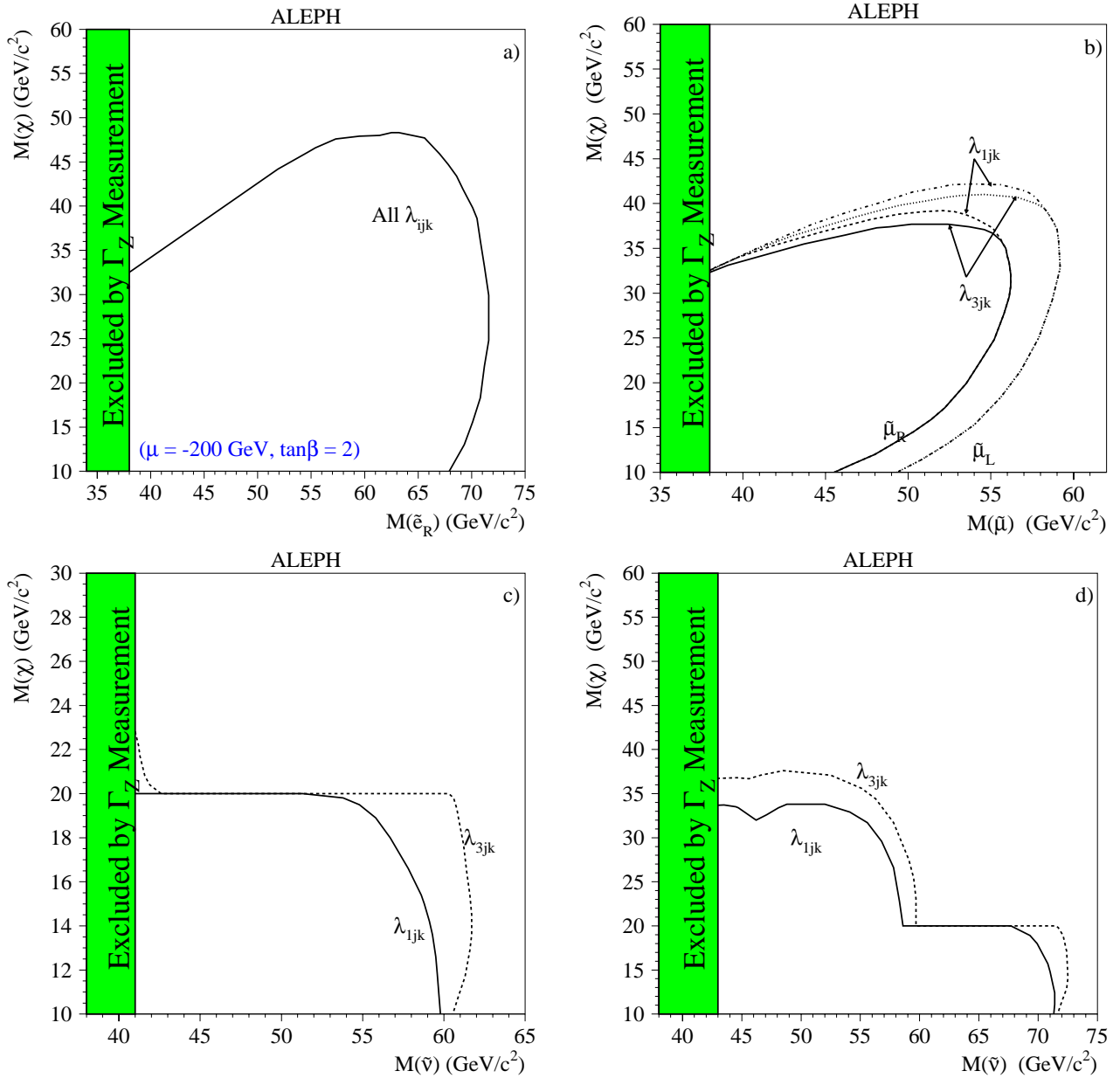
Fig. 11a–d. The 95% C.L. limits on the selectron, smuon and sneutrino in the (M_\chi, M_{\tilde{e}}) or (M_\chi, M_{\tilde{\nu}}) plane for the indirect decay modes. d shows the limit for three degenerate sneutrinos. The selectron cross section is evaluated at \mu = -200 GeV and \tan\beta = 2
