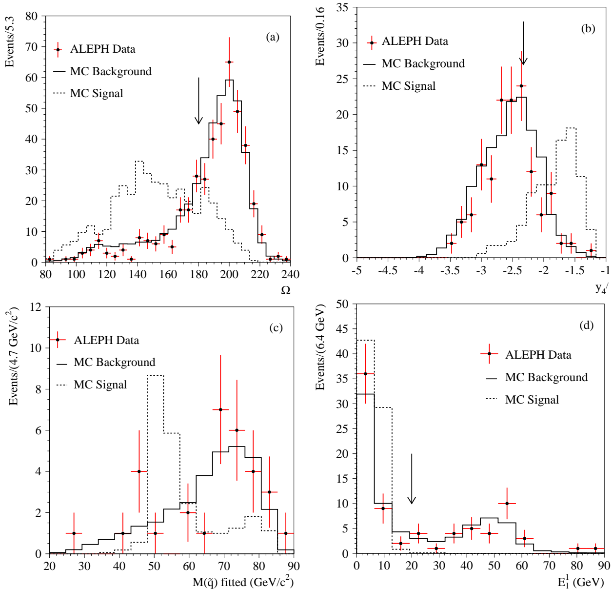
Fig. 2a–d. The distributions of a \Omega = \Phi'_{aco} + 0.7(M'_{vis} - 120) as used in subselection I of the “Multi-jets plus Leptons” selection, b the y'_4 variable as used in subselection II and III of the “Multi-jets plus Leptons” selection, c the reconstructed invariant mass M_{\bar{q}} as used in the “2J + 2 \tau ” selection, and d the energy of the leading lepton E_1^1 as used in the direct Chargino/Neutralino selections. The data (dots) at \sqrt{s} = 161\text{--}172 GeV are compared to the background Monte Carlo (full histograms). The dashed histograms show typical signal distributions for \lambda'_{3jk} in arbitrary normalisation: a and b \chi^+\chi^- \rightarrow W^*W^*\chi\chi , c t\bar{t} \rightarrow \tau q\tau q with M_{\bar{t}} = 50 GeV/ c^2 and d \chi^+\chi^- \rightarrow qq\tau qq\tau . In all cases only a subset of the cuts was applied to preserve sufficient statistics. Arrows indicate the cut positions
