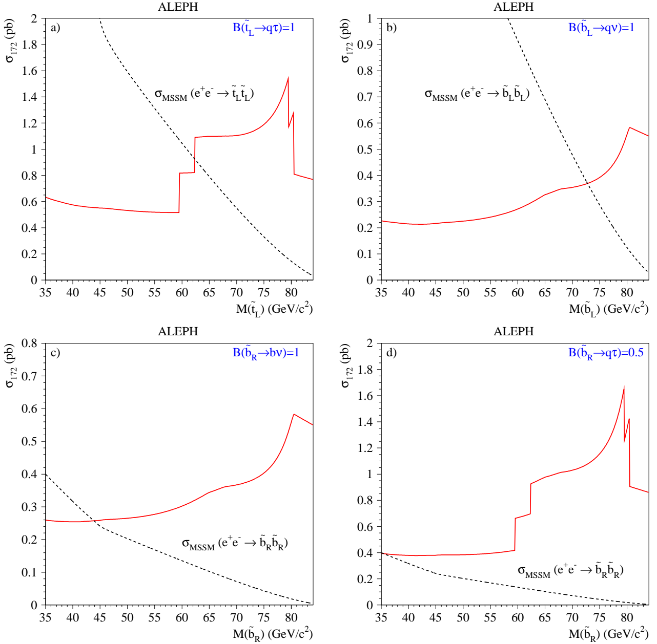
Fig. 12a–d. The 95% C.L. excluded cross sections for the direct decays of a \tilde{t}_L \tilde{t}_L \rightarrow \tau q \tau q , b \tilde{b}_L \tilde{b}_L \rightarrow q \nu q \nu , c \tilde{b}_R \tilde{b}_R \rightarrow b \nu b \nu and d \tilde{b}_R production with a 50% branching ratio into \tau q and \nu q . The MSSM cross sections are superposed as dashed lines
