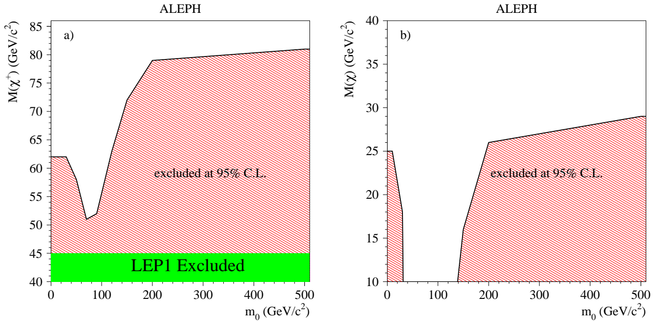
Fig. 9a,b. The limits on a the chargino mass and b the neutralino mass as functions of m_0 obtained by scanning the (\mu, M_2) plane at \tan\beta = \sqrt{2} , assuming a BR of 100% for the direct decay modes
