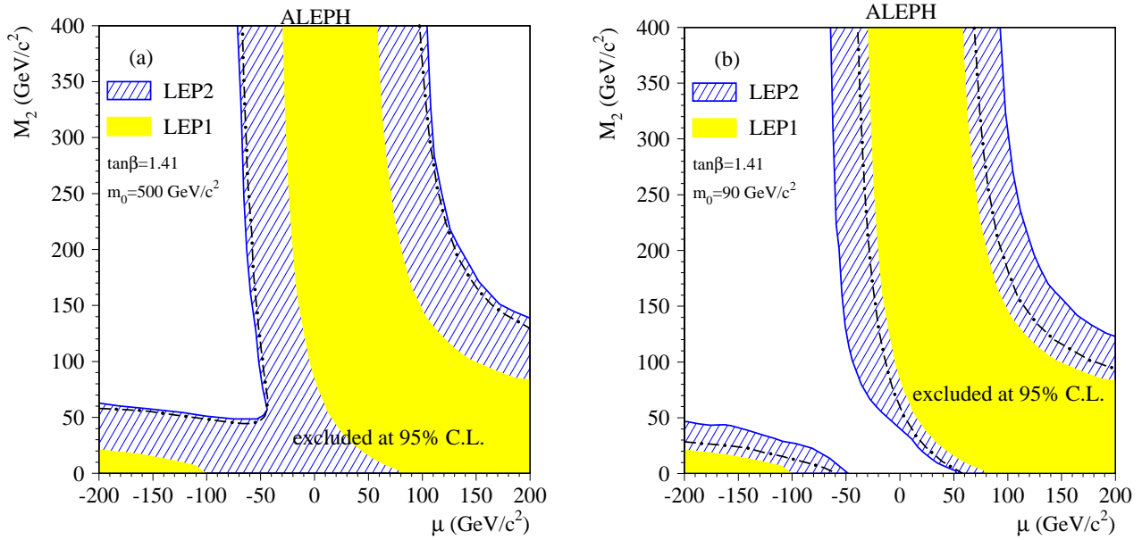
Fig. 8a,b. Regions in the (\mu, M_2) plane excluded at 95% C.L. at \tan\beta = \sqrt{2} assuming that charginos/neutralinos decay directly with a BR of 100%. a for m_0 = 500 \text{ GeV}/c^2 , where the inner dash-dotted lines show the overall chargino mass limit of M_{\chi^+} = 81 \text{ GeV}/c^2 . b for m_0 = 90 \text{ GeV}/c^2 , where the inner dash-dotted lines show the overall chargino mass limit of M_{\chi^+} = 52 \text{ GeV}/c^2
