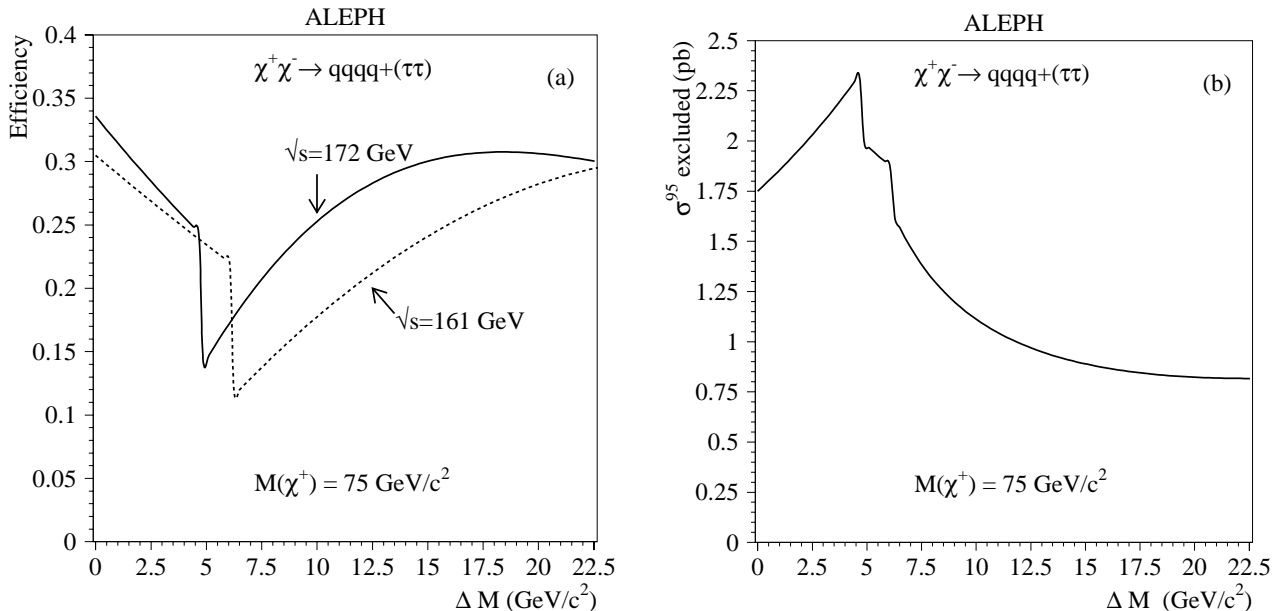
Fig. 7a,b. a The selection efficiencies for the direct chargino/neutralino decays \chi^+\chi^- \rightarrow 4q + 2\tau via two-body decays to sleptons/sneutrinos. Here \Delta M = M_{\chi^+} - M_{\tilde{\nu}} . For \Delta M \lesssim 5 GeV/c 2 the Four Jet selection is used, while for \Delta M \gtrsim 5 GeV/c 2 the 4J(2 \tau ) selection is used. b The corresponding 95% C.L. excluded cross section (at \sqrt{s} = 172 GeV)
