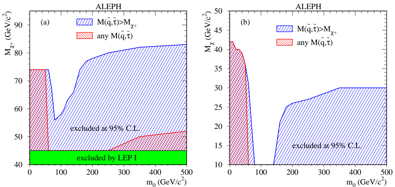
Fig. 4a,b. The limits on a the chargino mass and b the neutralino mass as functions of m_0 obtained by scanning the (\mu, M_2) plane at \tan\beta = \sqrt{2} , assuming a BR of 100% for the indirect decay modes
