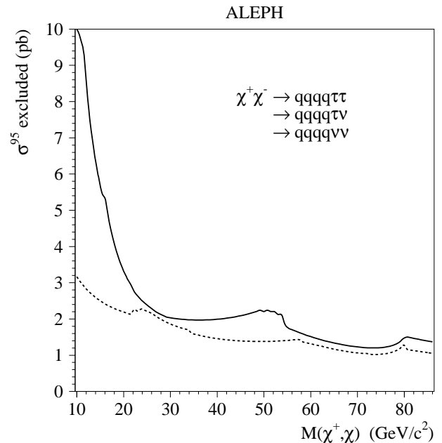
Fig. 6. The 95% C.L. limit on the chargino/neutralino cross section (at \sqrt{s} = 172 GeV) for direct three body decays of charginos/neutralinos and a non-zero coupling \lambda'_{3jk} . The dashed line corresponds to the most favourable chargino branching ratio, while the solid line corresponds to the worst case branching ratio. The latter is used to derive a conservative limit on the chargino/neutralino cross section
