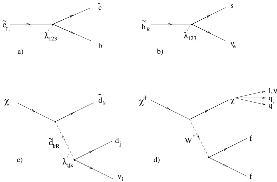
Fig. 1a–d. Examples of decays of supersymmetric particles: a direct decay of a left-handed selectron, b direct sbottom decay, c direct neutralino decay via sfermion exchange and d indirect chargino decay via exchange of a W^*
