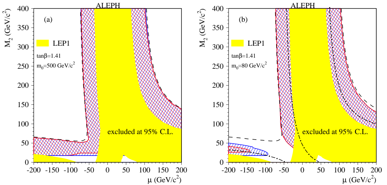
Fig. 3a,b. Regions in the (\mu, M_2) plane excluded at 95% C.L. at \tan\beta = \sqrt{2} and a m_0 = 500 \text{GeV}/c^2 or b m_0 = 80 \text{GeV}/c^2 , assuming that the indirect decays dominate (hatched regions). The white region below M_2 \lesssim 15 \text{GeV}/c^2 corresponds to neutralino masses less than 10 \text{GeV}/c^2 , the light shaded region to the LEP 1 limit. The superimposed dashed lines show the kinematic limit M_{\chi^+} = 86 \text{GeV}/c^2 . The dash-dotted line shows the M_{\chi^+} = 56 \text{GeV}/c^2 contour
