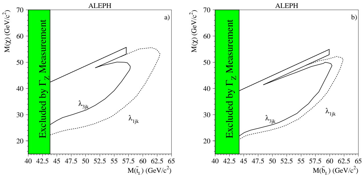
Fig. 13a,b. The 95% C.L. limits on the stop and sbottom in the (M_\chi, M_{\tilde{b}_L}) plane for the indirect decay modes. The limits are shown for the optimistic case of left-handed squarks
