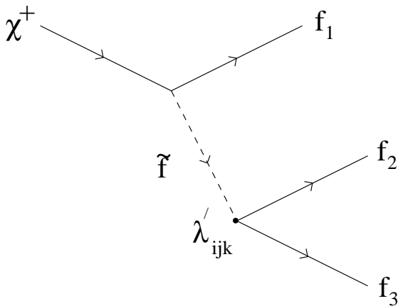
Fig. 5. Generic diagram for a direct chargino decay. The exchanged sfermion \tilde{f} may either be on-shell (2-body decay), or off-shell (3-body decay)
